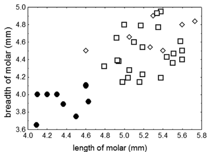
Fig. 2. Size distinction in the upper first molar (M1) in N. meridensis (closed symbols) and N. olivacea (open symbols). Symbols: Closed dots = N. meridensis (Venezuela); open squares = N. o. olivacea (Colombia); open diamonds = N. o. quitensis (Ecuador).
